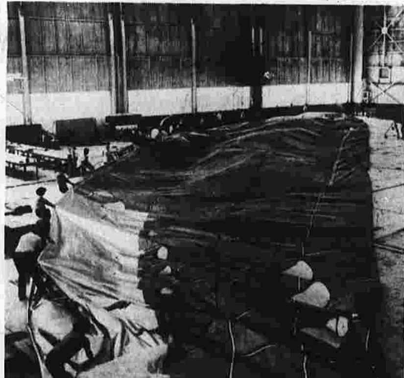
The America's envelope of neoprene-coated Dacron has been cut and stitched and is now ready for inflation.
